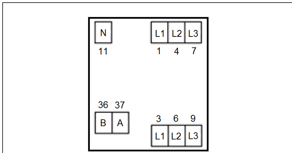
Abb. 6: Anschlüsse
